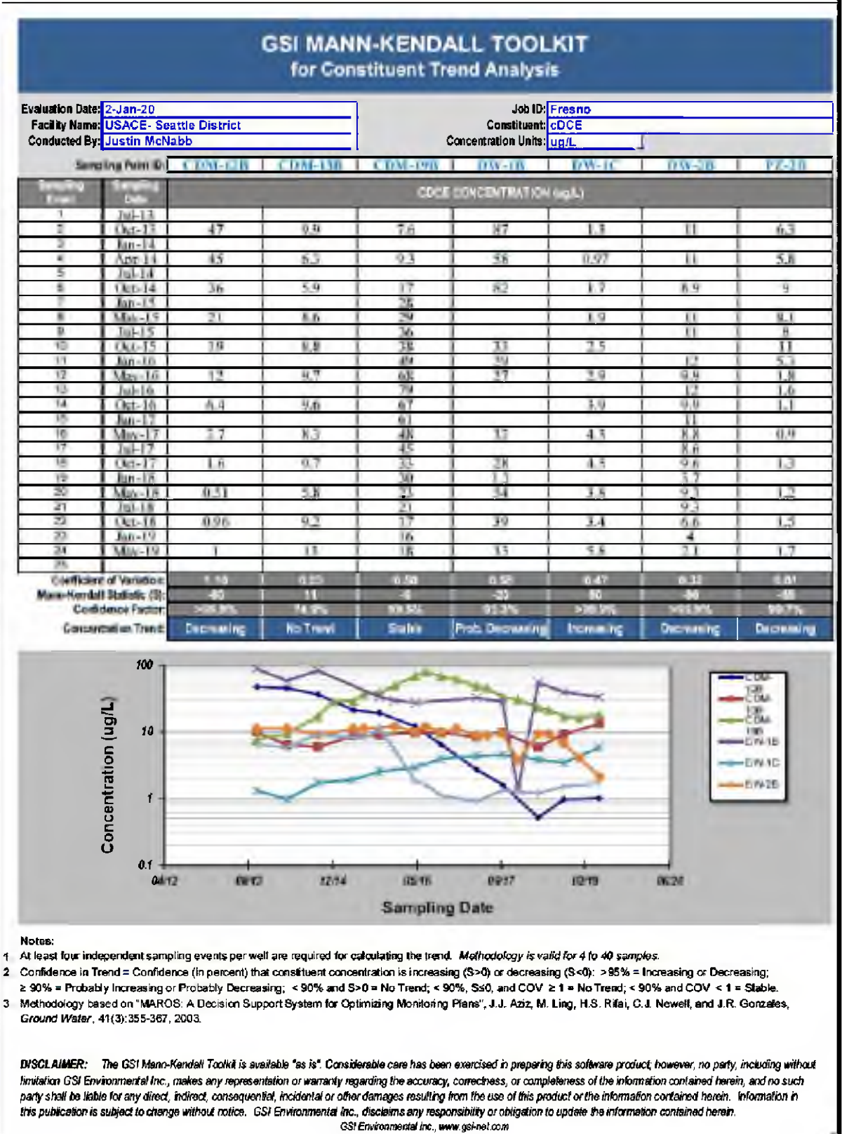
Figure C-2. Mann-Kendall trend analysis for cDCE in the B-zone aquifer. Three wells are above the MCL for cDCE but are stable or probably decreasing. One well is increasing but currently below the MCL.
