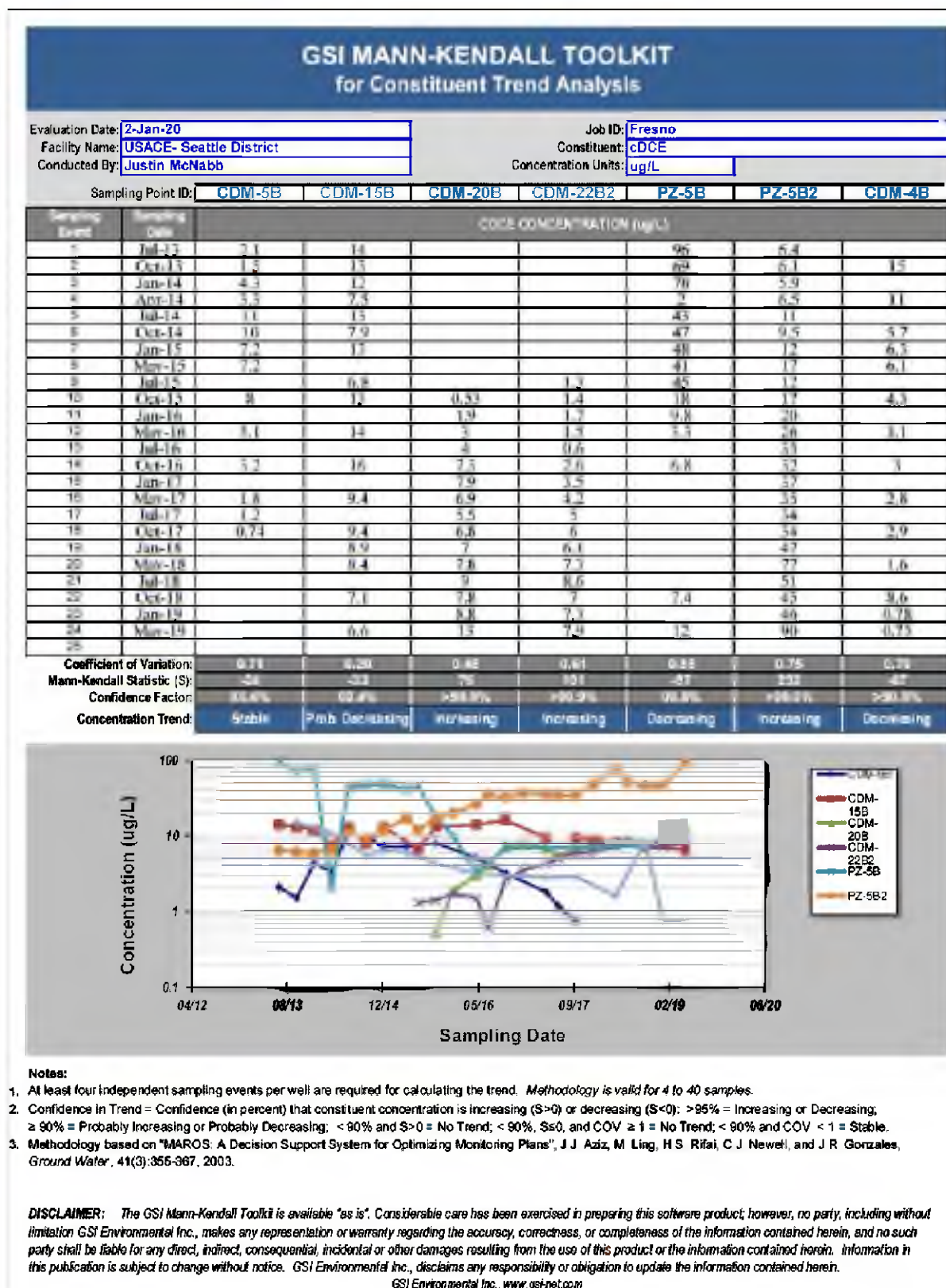
Figure C-1. Mann-Kendall trend analysis for cDCE in the B-zone aquifer with multiple increasing wells. All increasing wells are above the MCL for cDCE.
